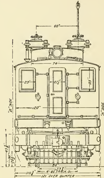
Fig. 268. End View of Great Northern Locomotive
